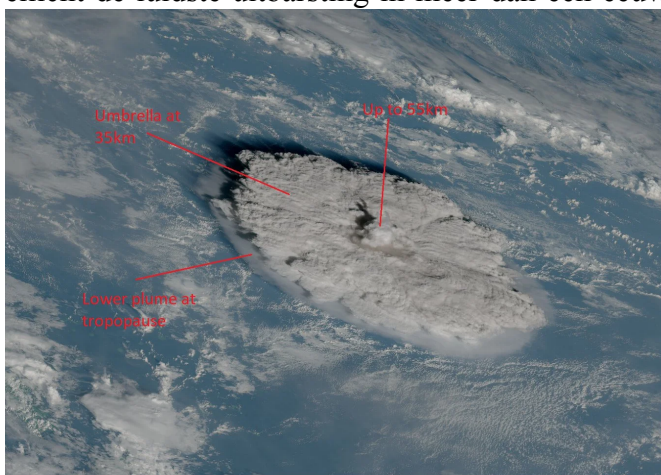
Image: @simon_sat / @nceoscience Data: Himawari-8 JMA
